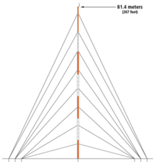
Figure 9. Example of a met tower.
