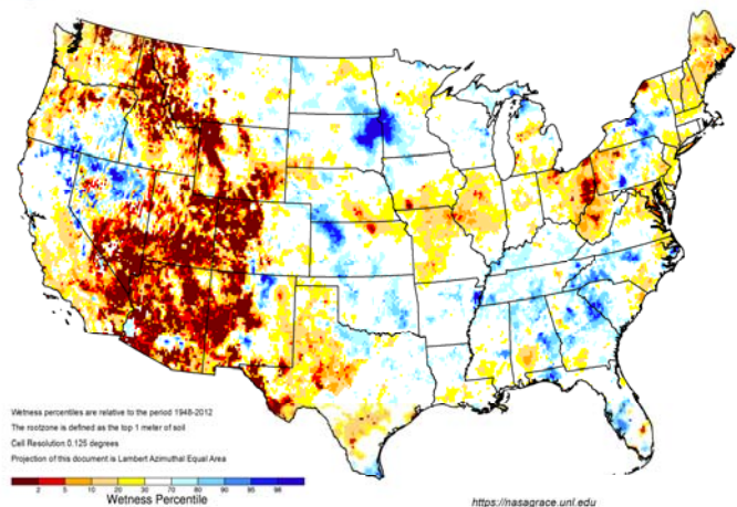
NASA GRACE-Based Root Zone Soil Moisture Drought Indicator August 25, 2025
