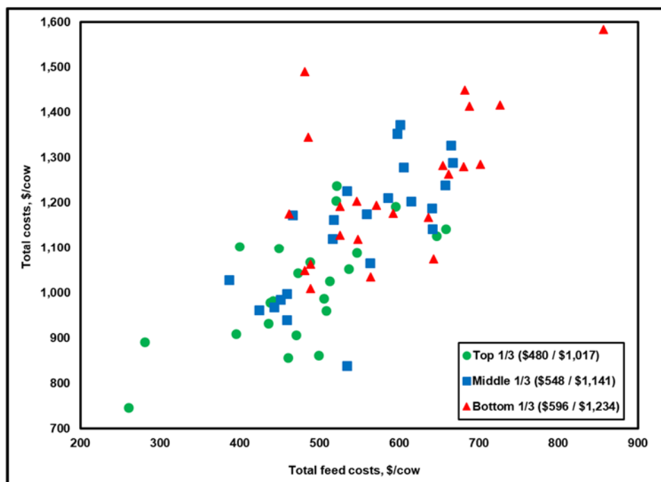
Figure A5. Total Costs vs. Total Feed Costs (correlation = 0.76)
