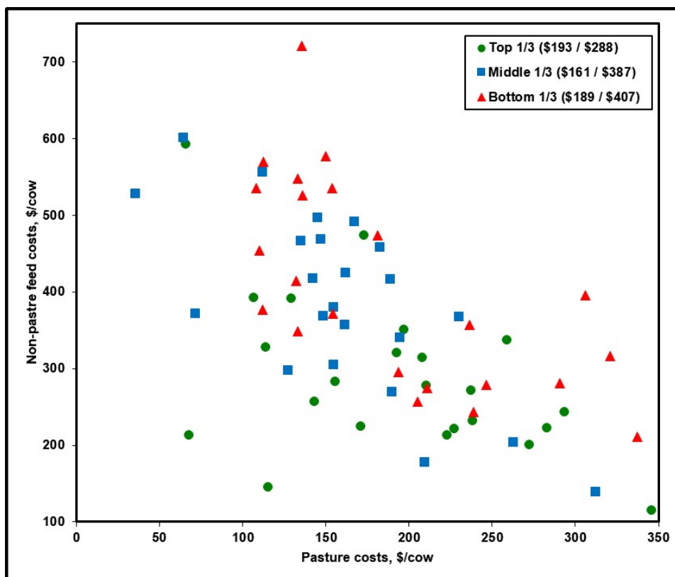
Figure A9. Non-Pasture Feed Costs vs. Pasture Costs (correlation = -0.60)
