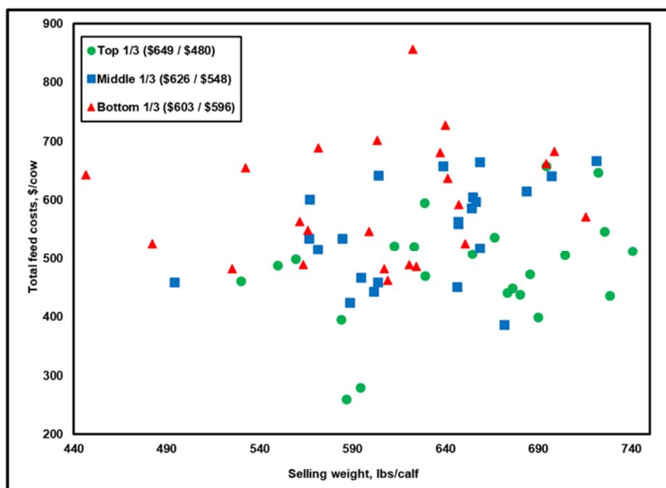
Figure A6. Total Feed Costs vs. Calf Selling Weight (correlation = 0.12)
