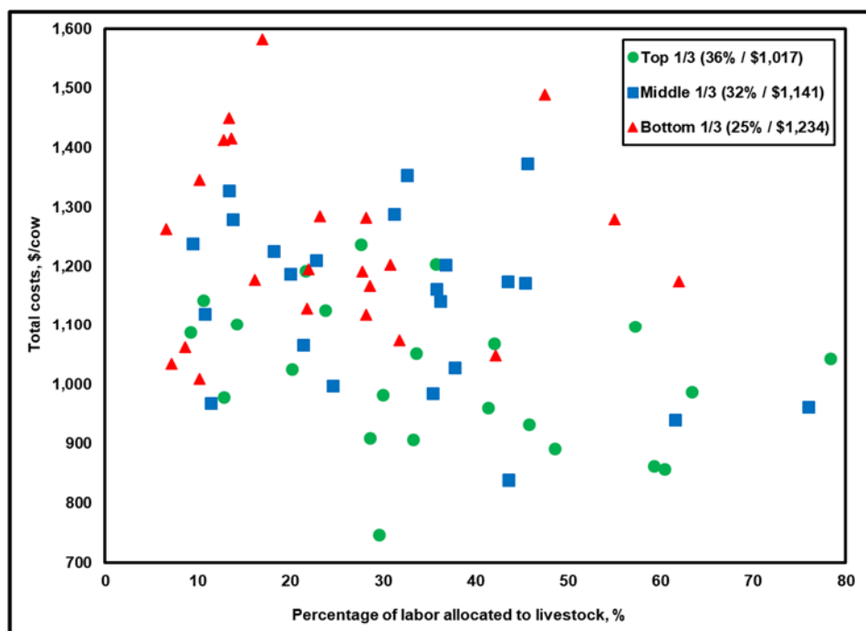
Figure A17. Total Costs vs. Labor Allocated to Livestock (correlation = -0.33)
