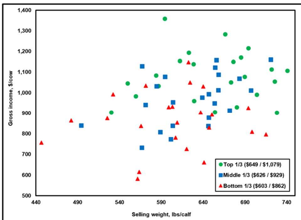
Figure A3. Gross Income vs. Calf Selling Weight (correlation = 0.33)
