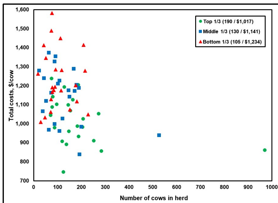
Figure A16. Total Costs vs. Size of Cow Herd (correlation = -0.37)
