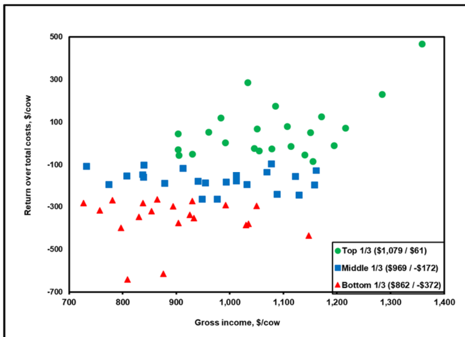
Figure A1. Profit vs. Gross Income (correlation = 0.60)
