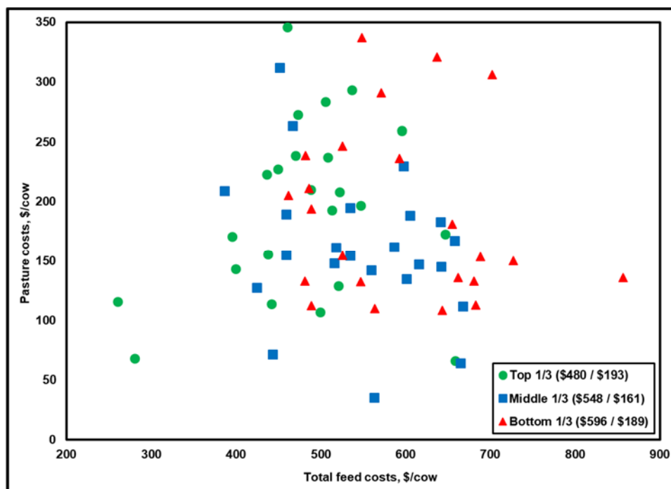
Figure A11. Pasture Costs vs. Total Feed Costs (correlation -0.07)
