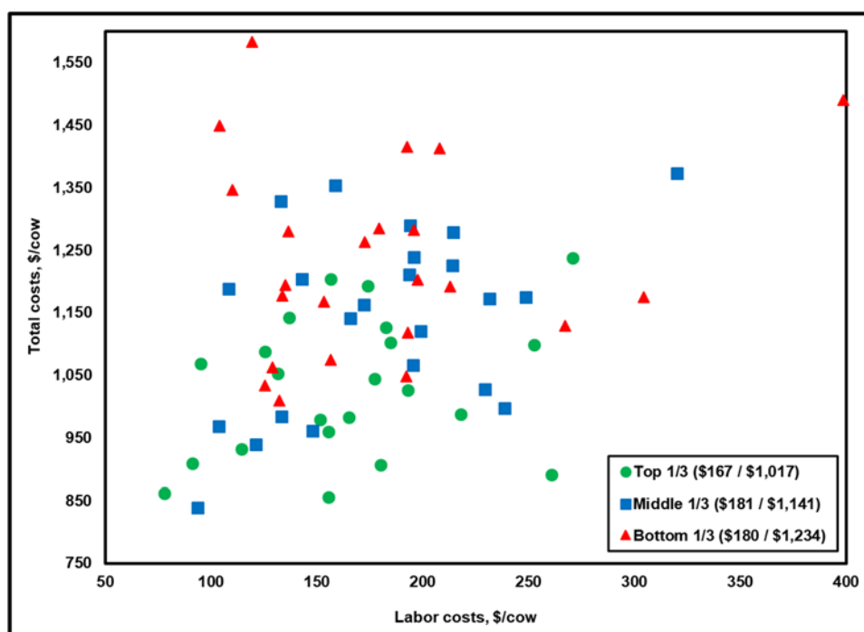
Figure A12. Total Costs vs. Labor Costs (correlation = 0.27)
