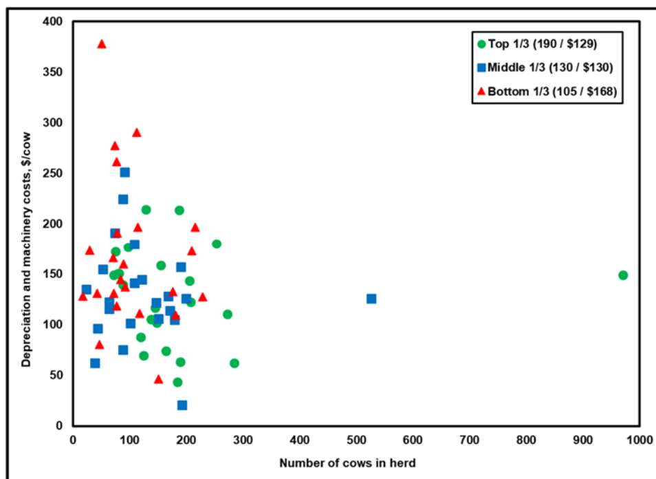
Figure A15. Depreciation and Machinery Costs vs. Size of Cow Herd (correlation = -0.12)
