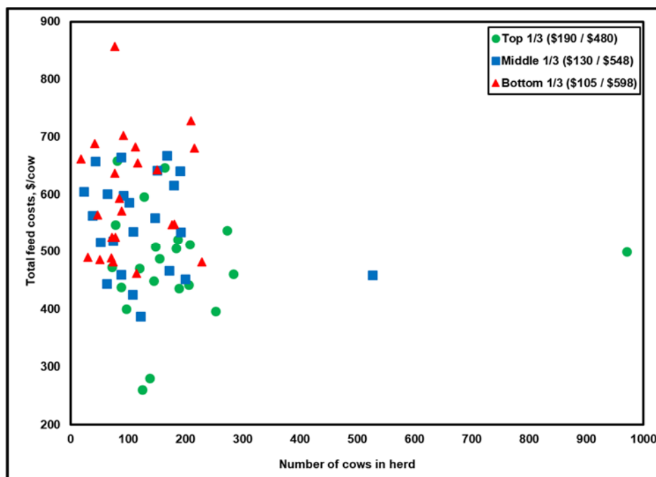
Figure A7. Total Feed Costs vs. Size of Cow Herd (correlation = -0.15)
