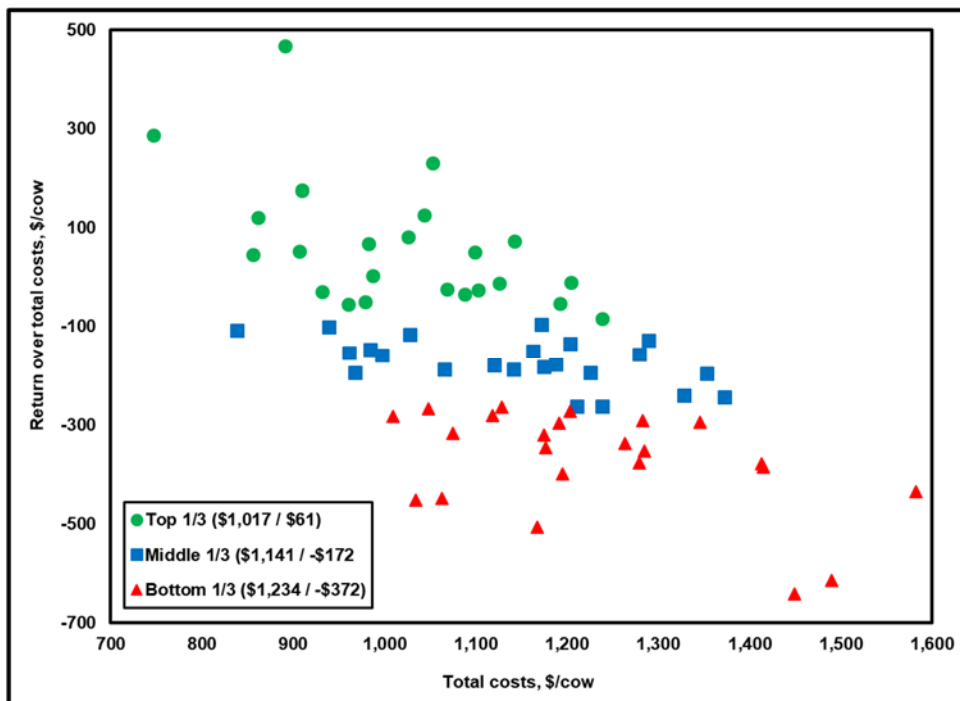
Figure A4. Profit vs. Total Costs (correlation = -0.66)
