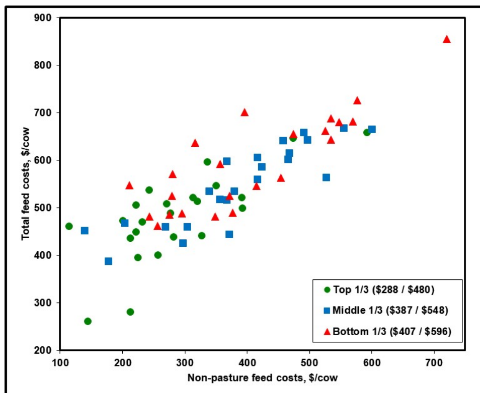
Figure A8. Total Feed Costs vs. Non-Pasture Feed Costs (correlation = 0.84)
