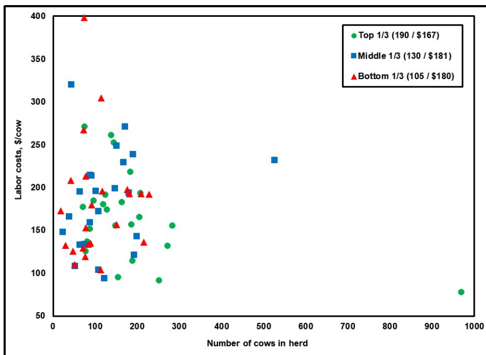
Figure A13. Labor Costs vs. Size of Cow Herd (correlation = -0.29)
