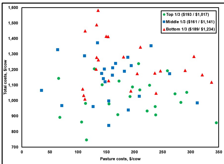
Figure A10. Total Costs vs. Pasture Costs (correlation = -0.09)
