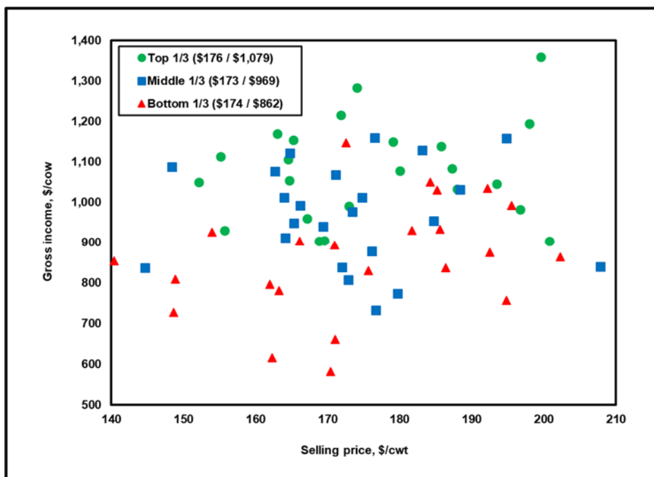
Figure A2. Gross Income vs. Selling Price (correlation = 0.18)
