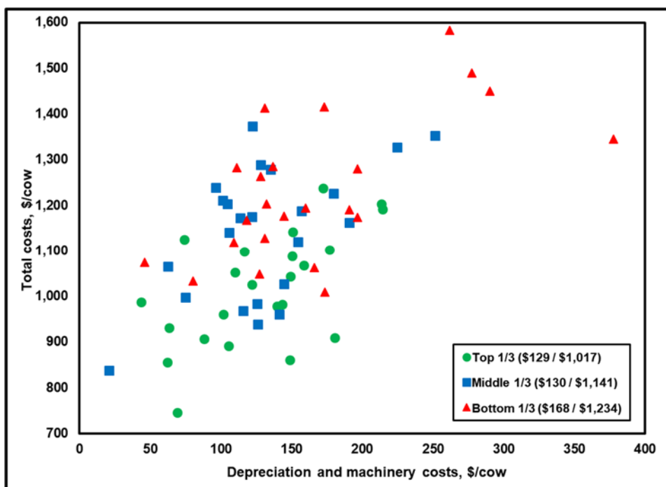
Figure A14. Total Costs vs. Depreciation and Machinery Costs (correlation = 0.61)
