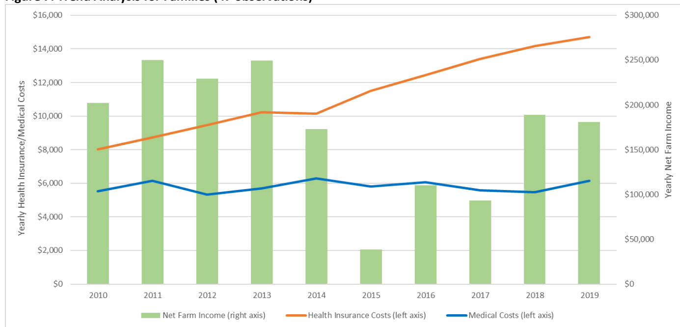
Figure 7: Trend Analysis for Families (47 observations)
