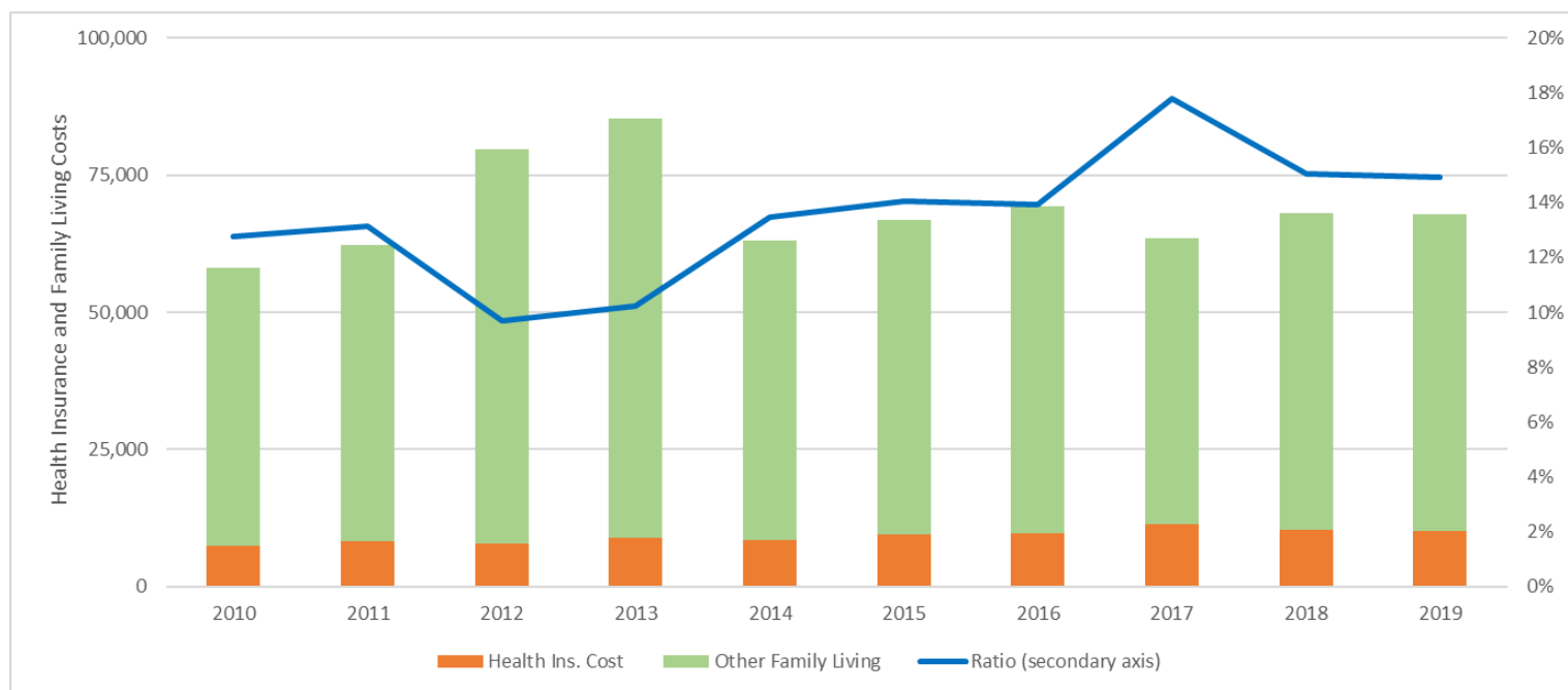
Figure 9: Trends in Health Insurance and Total Family Living Expense for Couples >65 Years of Age (15 observations)
