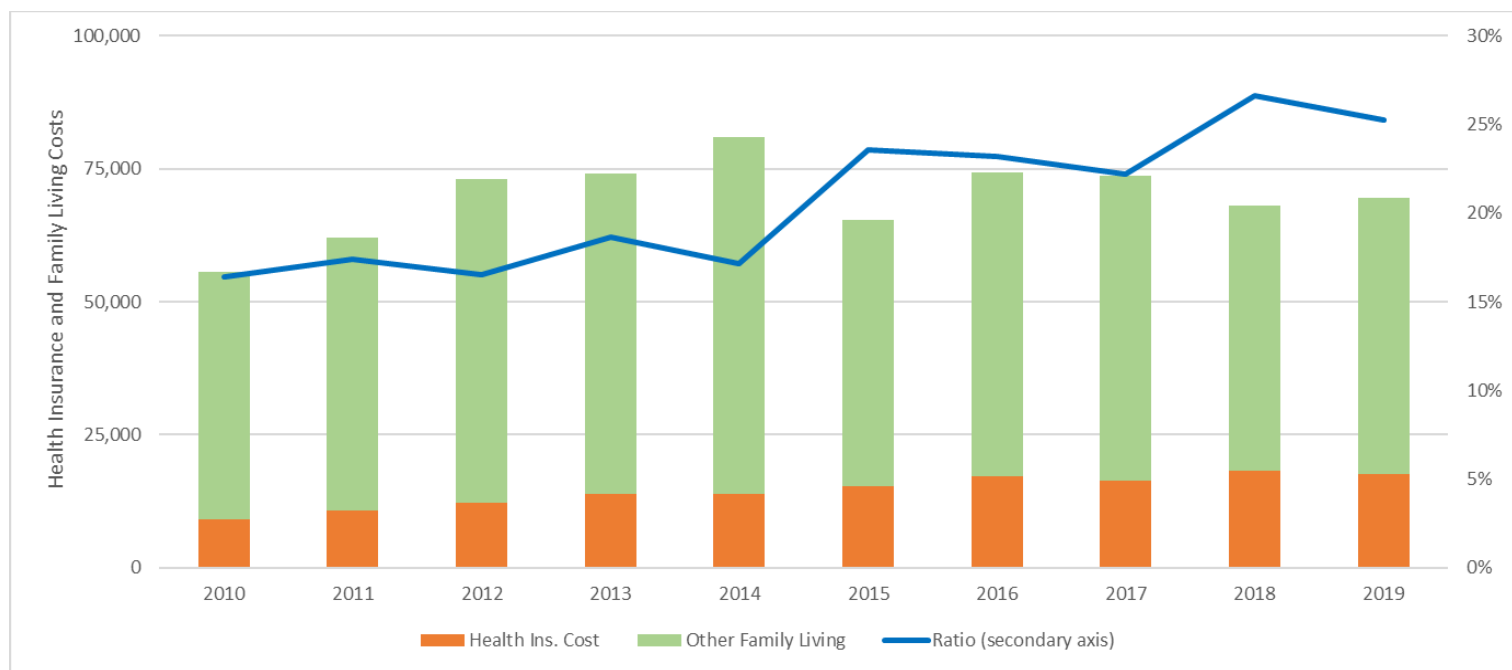
Figure 8: Trends in Health Insurance and Total Family Living Expense for Couples <65 Years of Age (14 observations)
